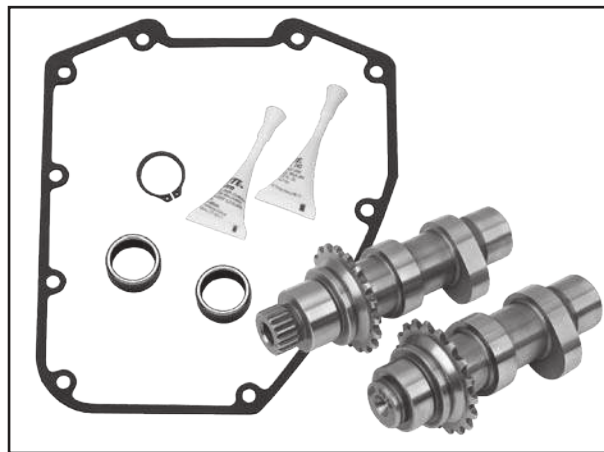
Complete Chain Drive Camshaft Kit
